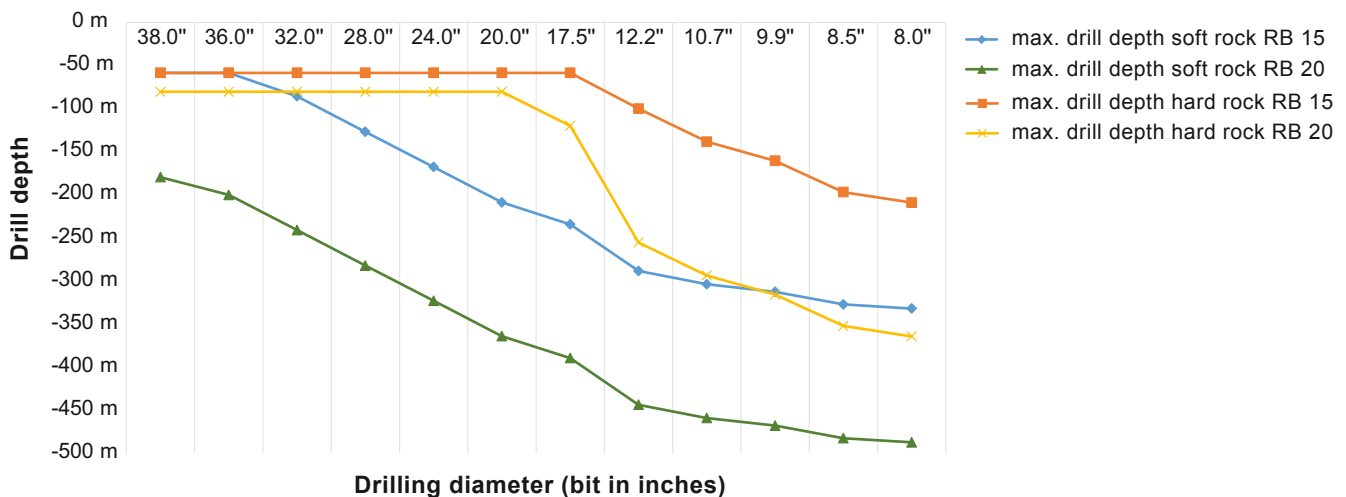
RB 15 / RB 20: max. drilling depths with 5.1/2 IF DP, incl. DC
